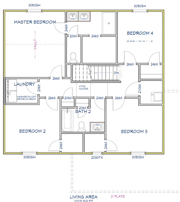
Second Level
