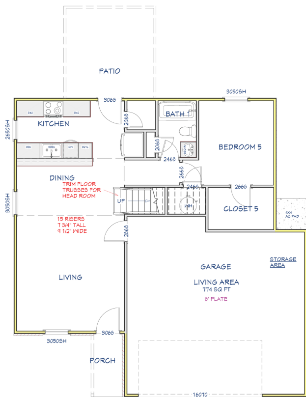
Main Level
